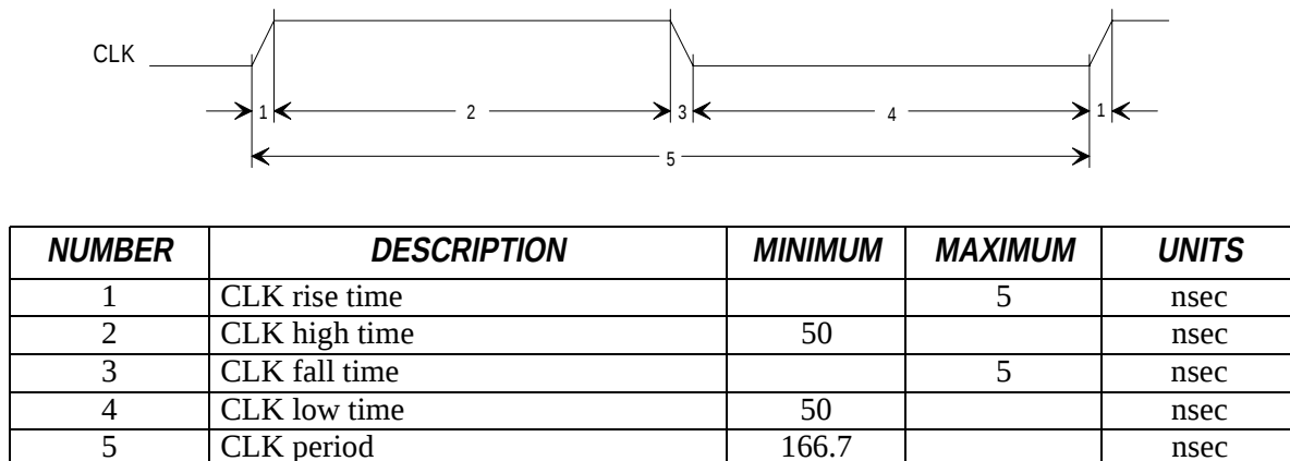
Figure 7: CLK Characteristics
