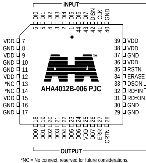
Figure 3: Pinout
