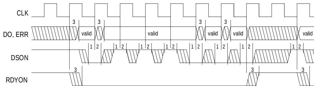
Figure 11: Data Output
