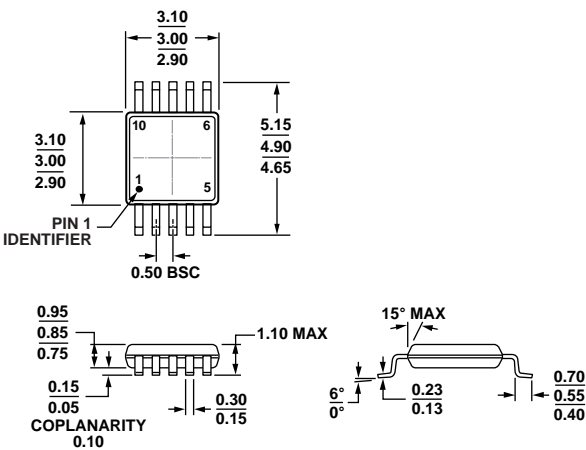
COMPLIANT TO JEDEC STANDARDS MO-187-BA Figure 30. 10-Lead Mini Small Outline Package [MSOP] (RM-10) Dimensions shown in millimeters
