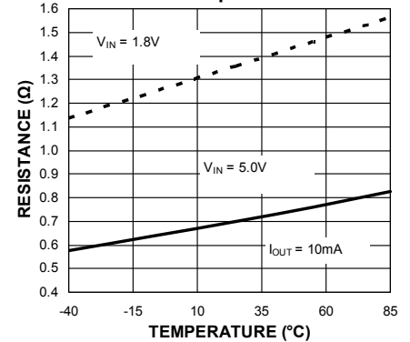
R_{DS(ON)} vs. Temperature
