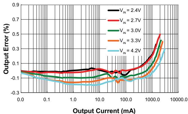
Load Regulation (L = 2.2μH, V OUT = 5.0V)
