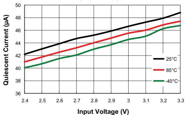
No Load Quiescent Current vs Input Voltage (Open Loop)
