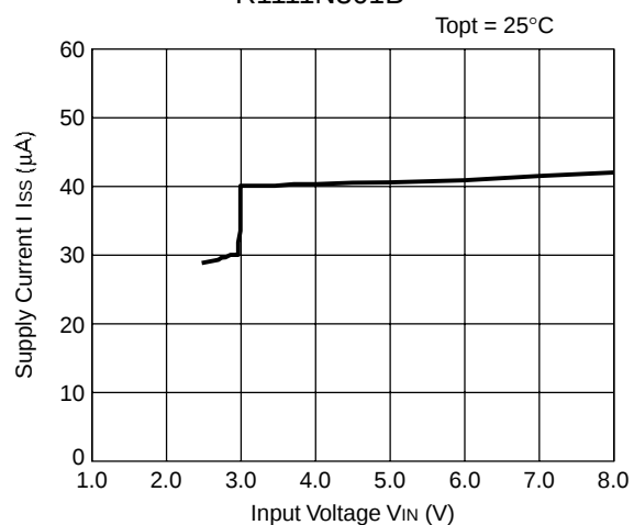
R1111N301B
