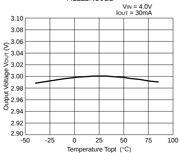
R1111N301B
