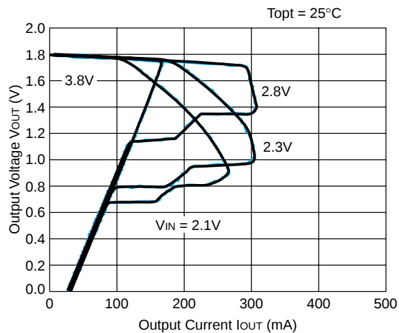
R1111N181B
