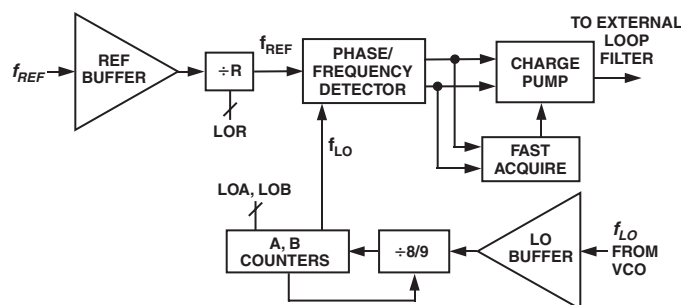
Figure 5. LO Synthesizer
