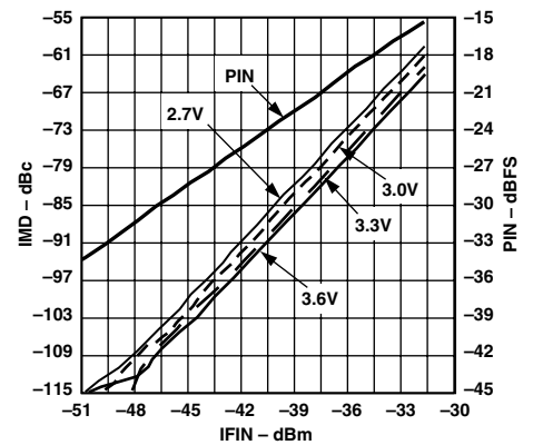
TPC 9c. IMD vs. IFIN (Low Bias 3 )
