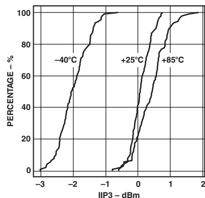
TPC 2a. CDF of IIP3 ( V_{DDx} = 3.0\text{ V} , High Bias 2 )
