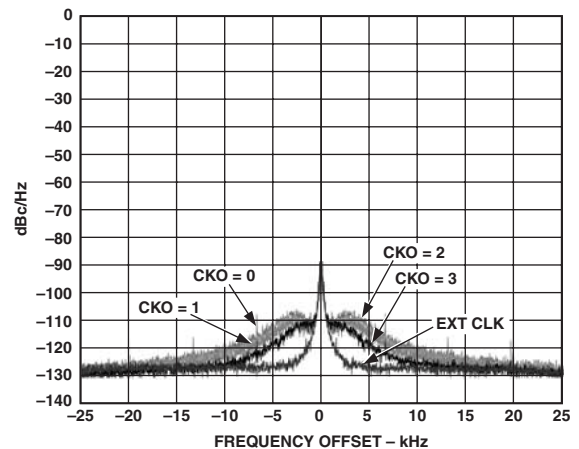
Figure 7b. CLK Phase Noise vs. I_{BIAS} Setting ( CKO ) ( IF = 73.35 \text{ MHz} , IF = 71.1 \text{ MHz} , IFIN = -31 \text{ dBm} , f_{CLK} = 18 \text{ MHz} , f_{REF} = 16.8 \text{ MHz} ) (CLK SYN Settings: CKI = 7 , CLR = 56 , and CLN = 60 with f_{REF} = 300 \text{ kHz} )
