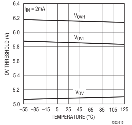
OV Threshold vs Temperature
