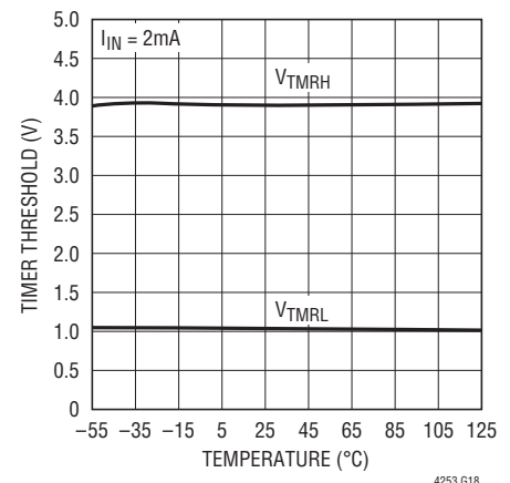
TIMER Threshold vs Temperature
