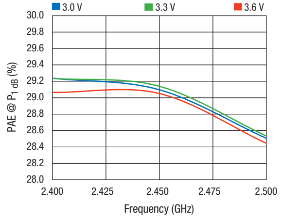
Figure 10. PAE @ P1dB vs Frequency Across VCC
