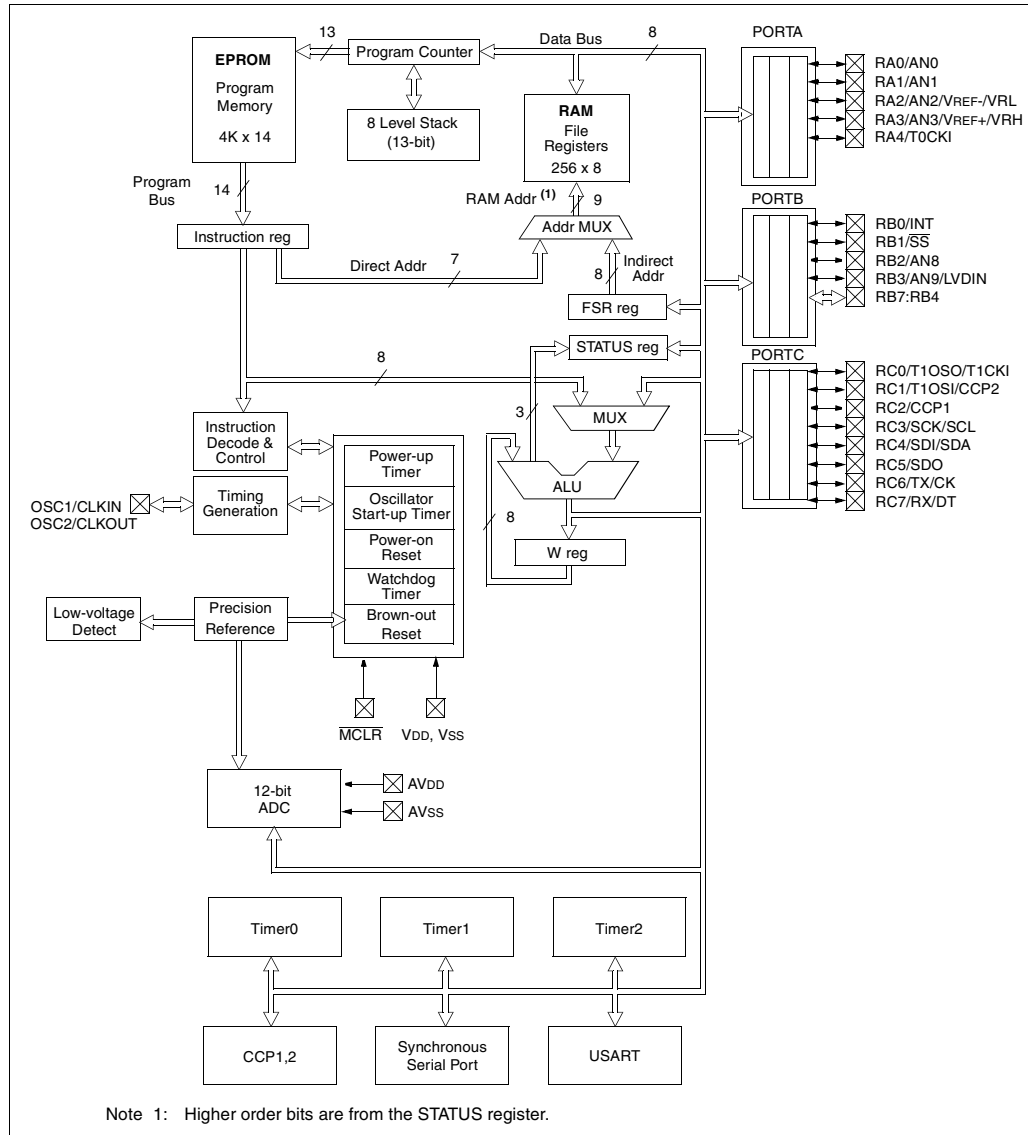
FIGURE 1-1: PIC16C773 BLOCK DIAGRAM
