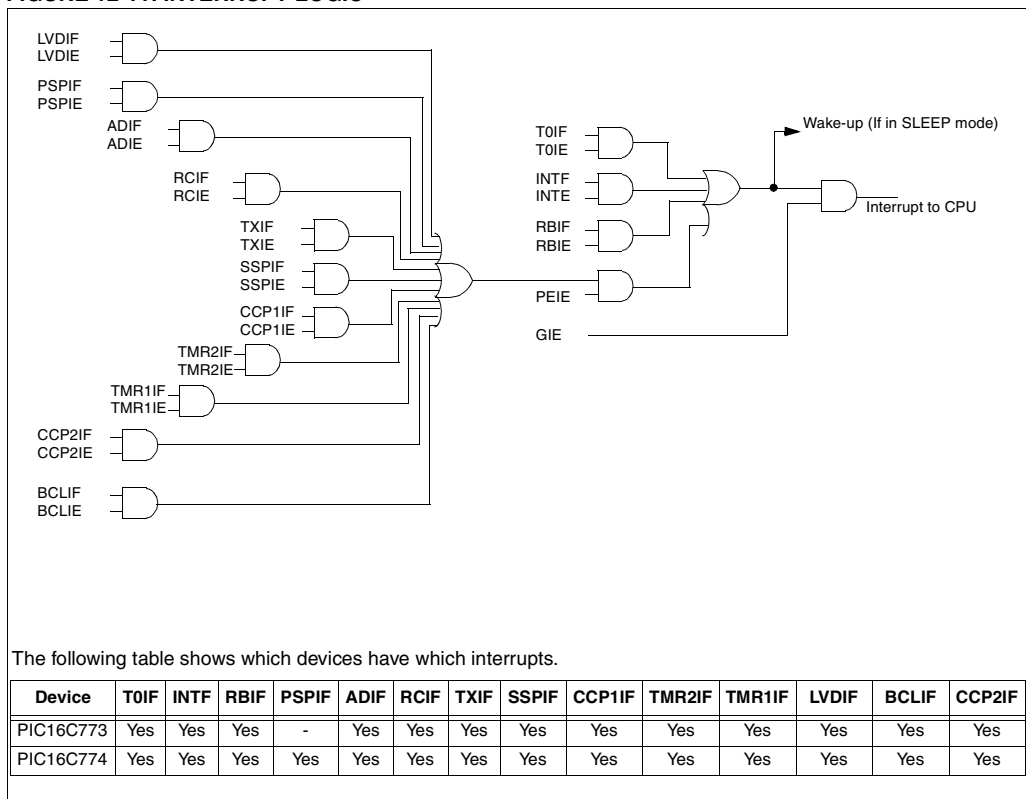
FIGURE 12-11: INTERRUPT LOGIC
