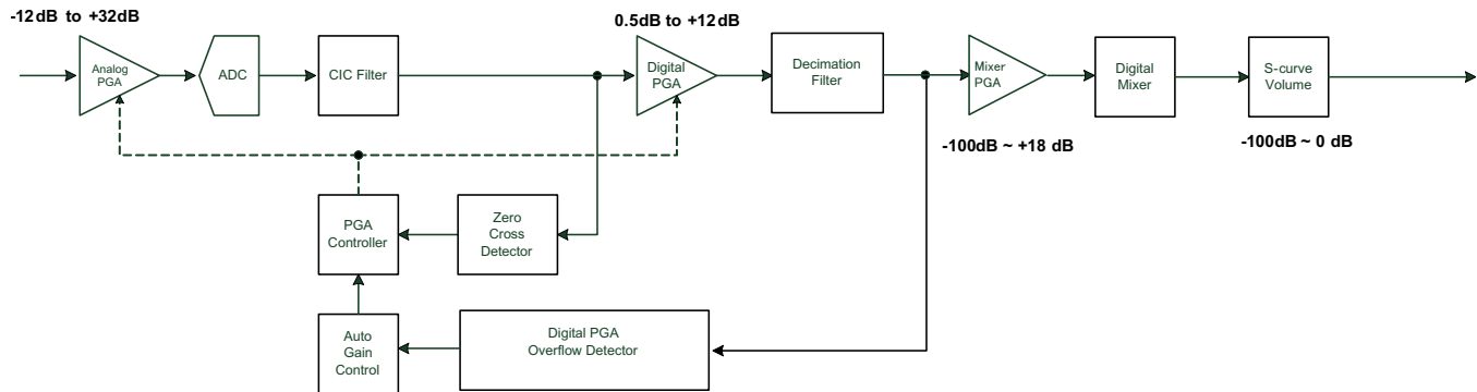
Figure 25. Sampling points within the PCM186x for Auto Clipping Suppression
