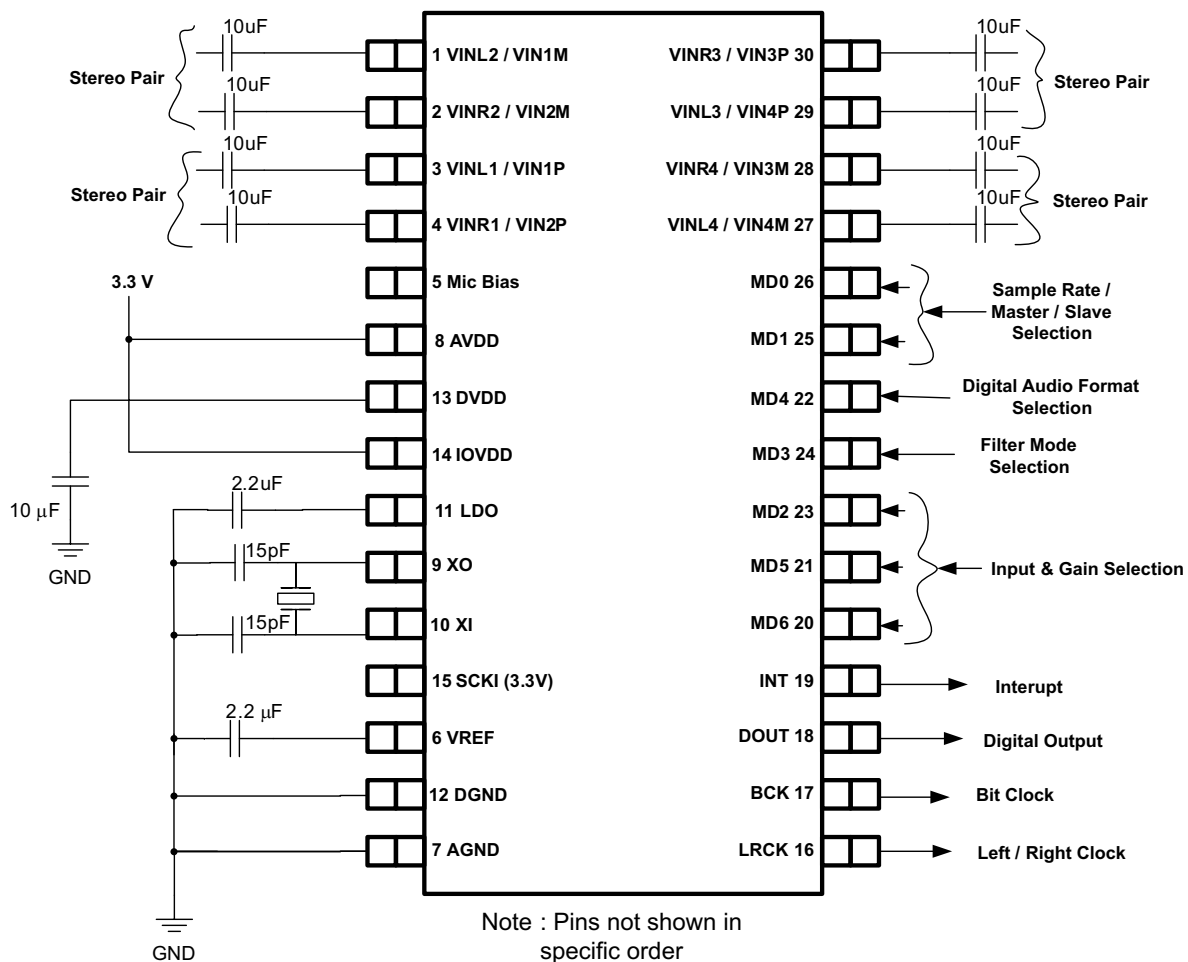
Figure 56. Simplified Schematic, PCM1861 Hardware-Controlled Subsystem
