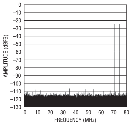
64k Point 2-Tone FFT, f_{IN} = 70.25\text{MHz} and 74.3\text{MHz} , -25\text{dBFS} , PGA = 0
