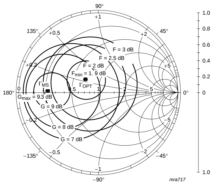
Fig 12. Noise circle figure; f = 2000 \text{ MHz} .
