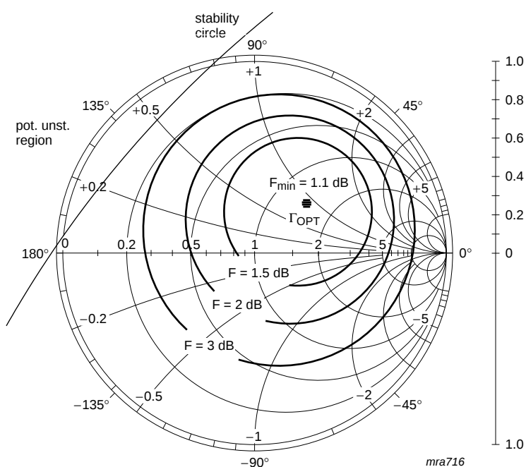
Fig 11. Noise circle figure; f = 900 \text{ MHz} .
