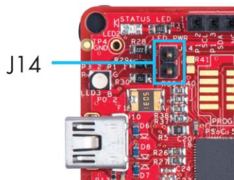
Figure 2-13: Remove J14 from CY8CKIT-040
