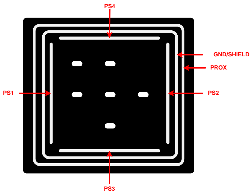
Figure 2-7: Sensor Pattern
