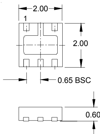
6 Pin SLP package (Bottom Side View) Nominal Dimensions in mm
