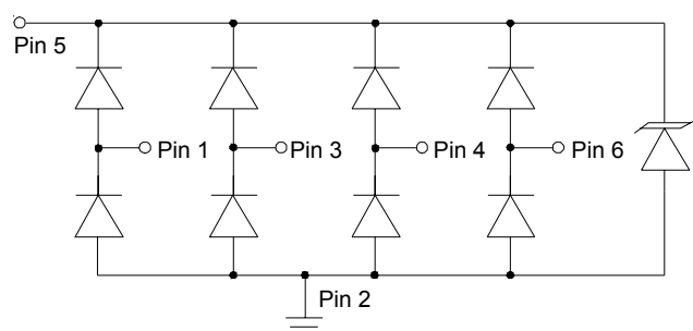
Device Schematic
