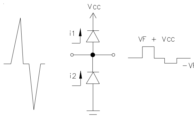
Figure 1 - "Rail-To-Rail" Protection Topology (First Approximation)
