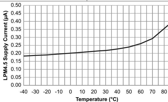
Figure 5-3. LPM4.5 Supply Current vs Temperature
