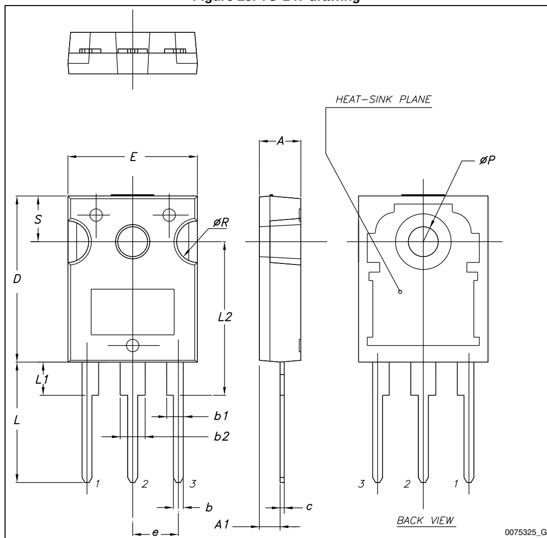
Figure 25. TO-247 drawing
