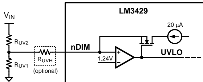
Figure 25. UVLO Circuit
