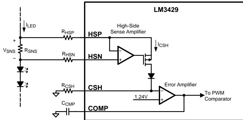
Figure 17. LED Current Sense Circuitry
