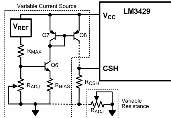
Figure 18. Analog Dimming Circuitry
