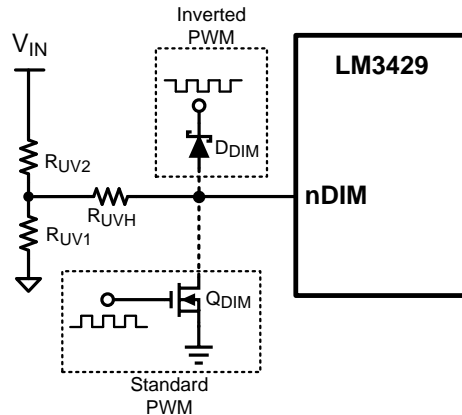
Figure 26. PWM Dimming Circuit
