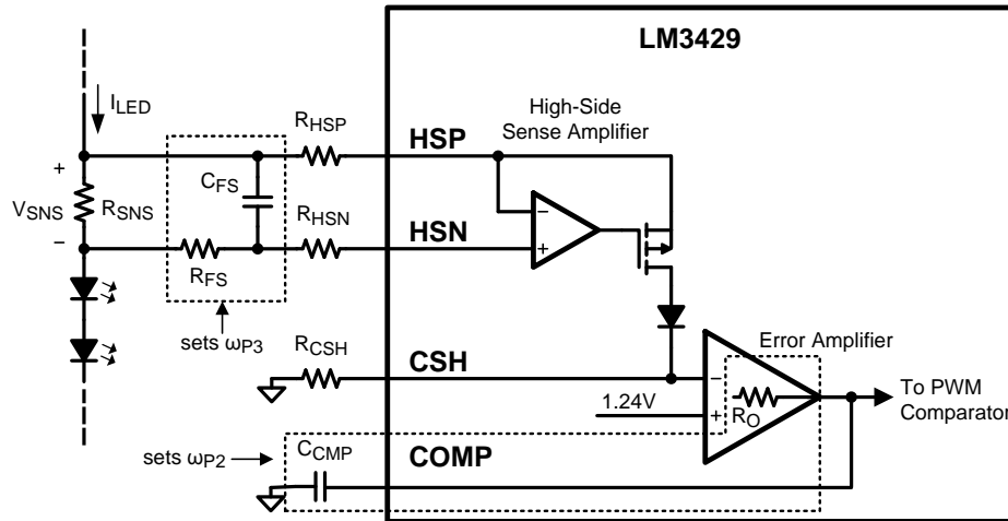
Figure 21. Compensation Circuitry
