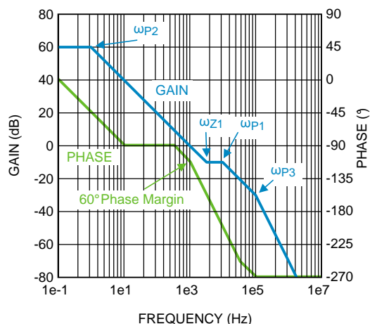
Figure 22. Compensated Loop Gain Frequency Response
