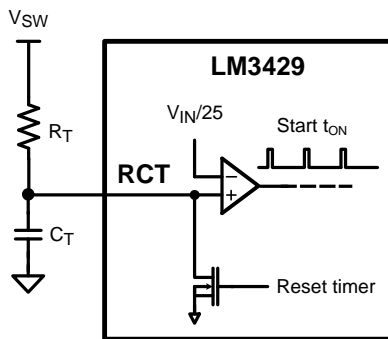
Figure 15. Off-timer Circuitry for Boost and Buck-boost Regulators
