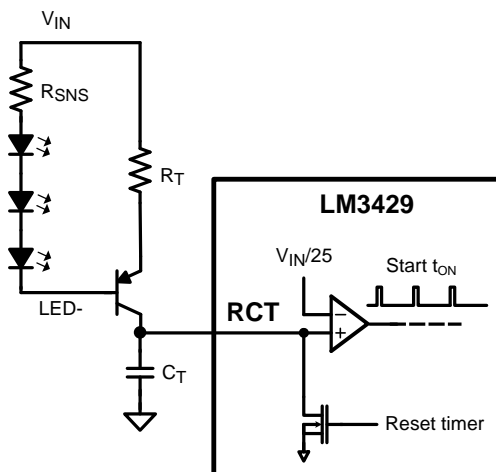
Figure 16. Off-timer Circuitry for Buck Regulators
