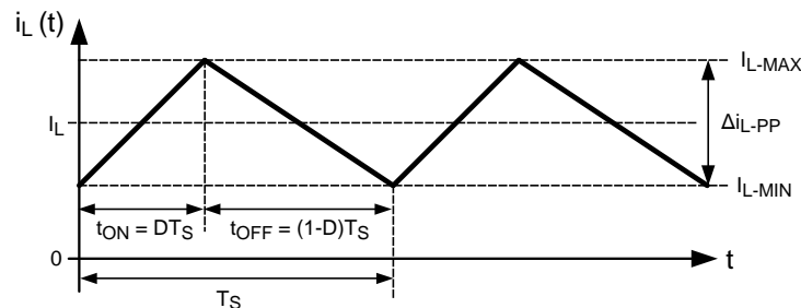
Figure 14. Ideal CCM Regulator Inductor Current i_L(t)
