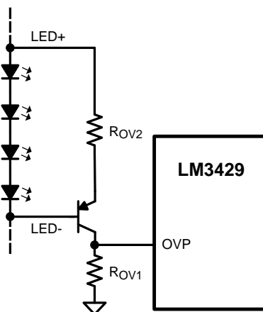
Figure 24. Floating Output OVP Circuitry
