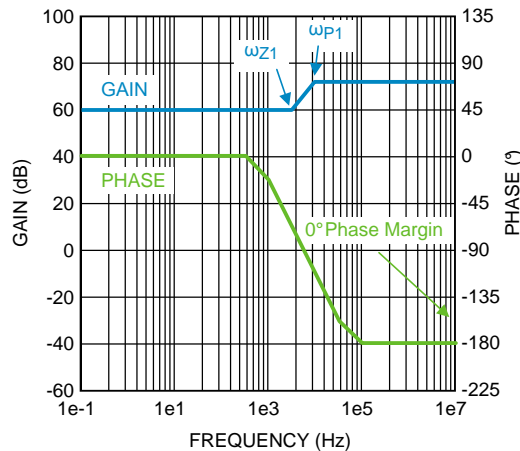
Figure 20. Uncompensated Loop Gain Frequency Response
