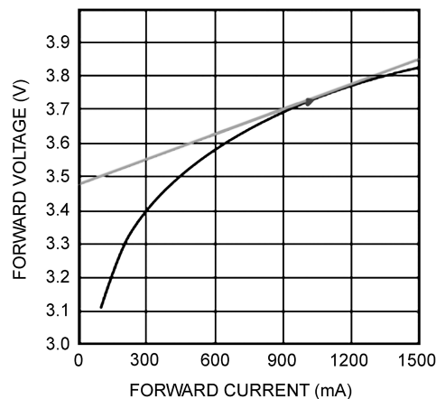
Figure 27. Dynamic Resistance
