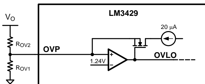
Figure 23. Over-Voltage Protection Circuitry
