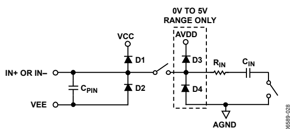
Figure 28. Simplified Analog Input
