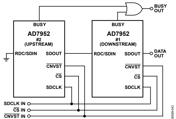
Figure 42. Two AD7952 Devices in a Daisy-Chain Configuration
