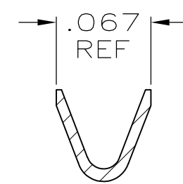
WIRE SIZE #22-#26 SECTION E-E
