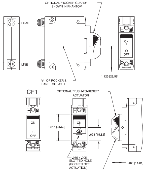
ROCKER SHROUDED ON "OFF" POSITION SIDE, SHOWN IN DASHED LINES.
