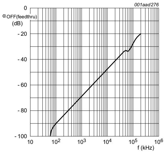
Fig 14. Switch OFF-state signal feed-through as a function of frequency
