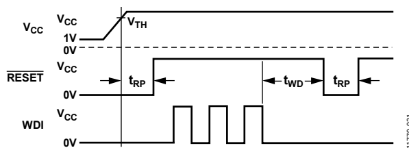
Figure 21. Watchdog Timing Diagram
