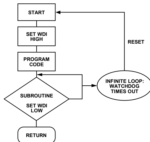
Figure 23. Watchdog Flow Diagram
