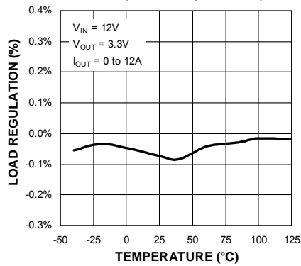
Load Regulation vs. Temperature (MIC2101)
