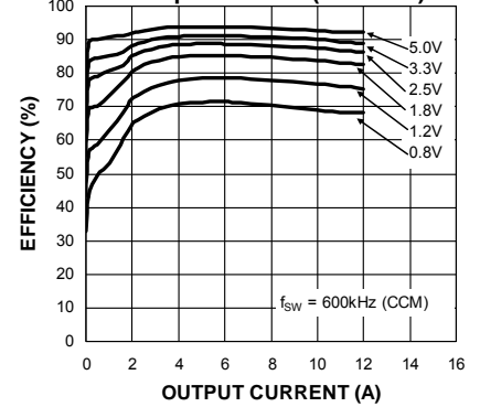
Efficiency ( V_{IN} = 12V ) vs. Output Current (MIC2101)
