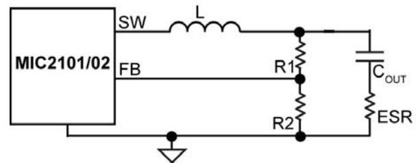
Figure 8a. Enough Ripple at FB
