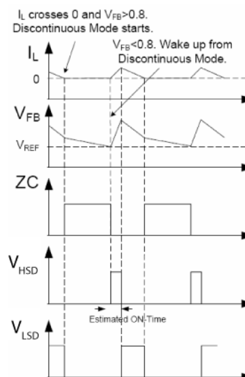
Figure 3b. MIC2101 Control Loop Timing (Discontinuous Mode)
