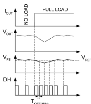
Figure 3a. MIC2101/02 Load Transient Response
