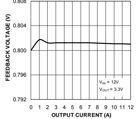
Feedback Voltage vs. Output Current (MIC2101)
