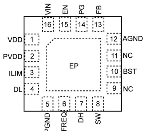
16-Pin 3mm x 3mm MLF (ML)
