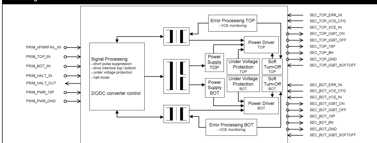
Block diagram
