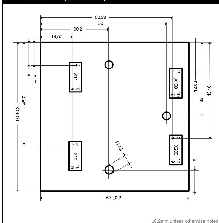
Dimensions in mm (bottom view)
