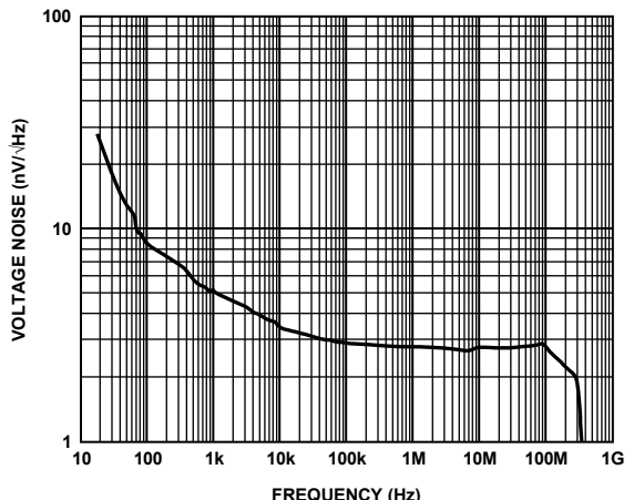
Figure 11. Voltage Noise vs. Frequency
