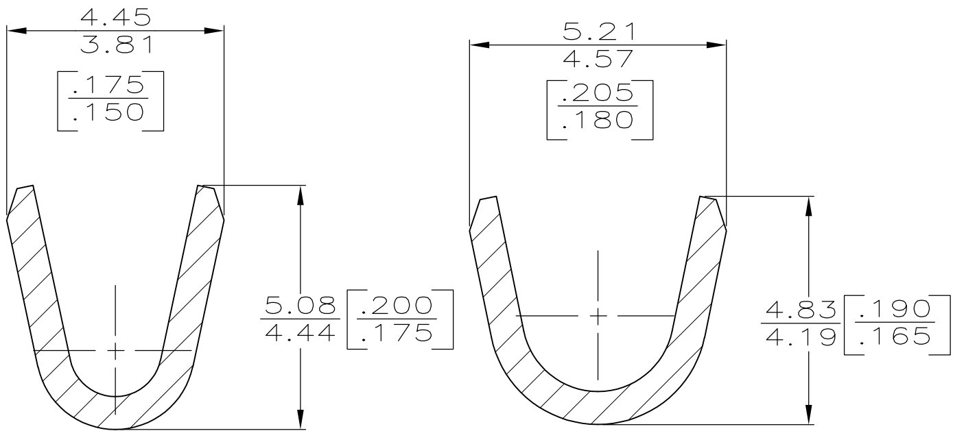
SECTION A—A SCALE 10:1
