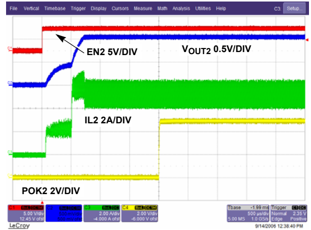
FIGURE 58. START-UP V_{OUT1} = 1.05V (FULL LOAD, PWM MODE)
