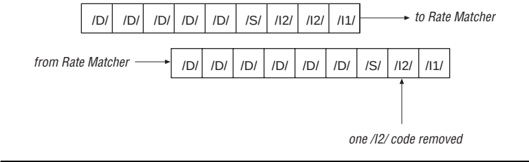
Figure 6–10. Detection of an /I2/ Ordered Set During an Almost Full Condition
