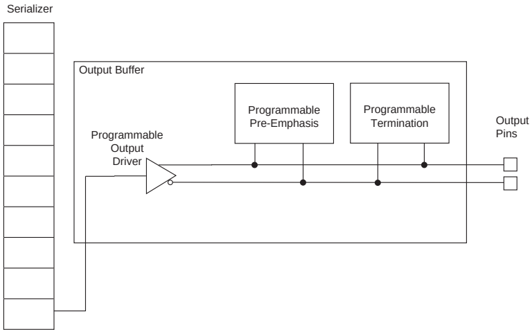
Figure 2–6. Output Buffer
