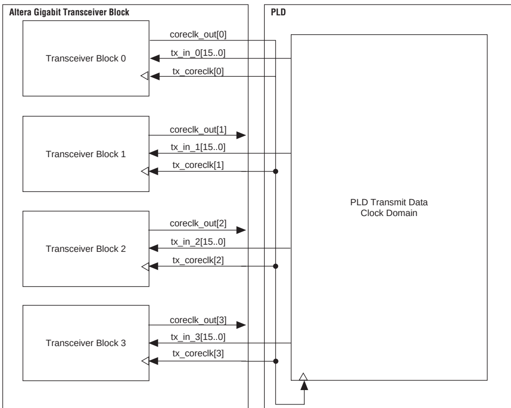
Figure 3–22. Example of a Multi-Transceiver Block Device to Transmitter Interface Clocking Scheme in Custom Mode
