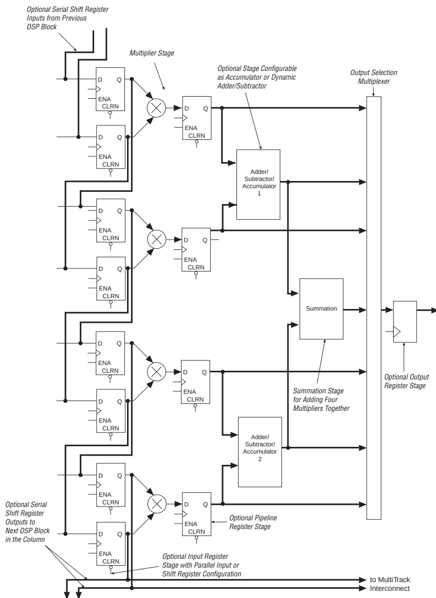
Figure 4–29. DSP Block Diagram for 18 \times 18 -Bit Configuration
