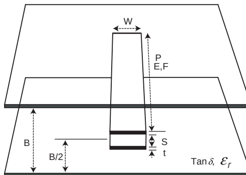
Figure 4–32. Broadside-Coupled Differential Stripline
