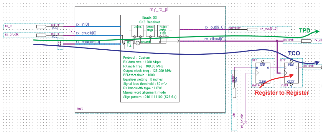
Figure 5–2. Receiver PLL rx\_clkout Showing t_{PD} & t_{CO} Registers
