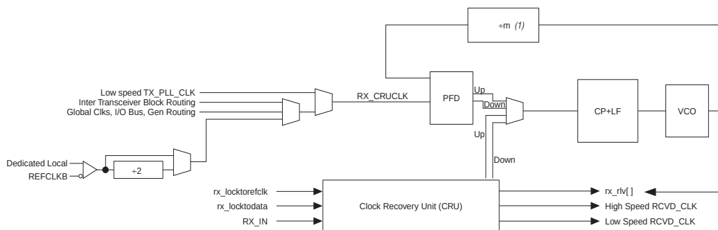
Figure 2–10. Receiver PLL Block Diagram
