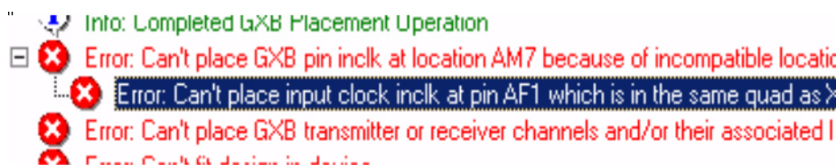
Figure 12–2. Error Messages
