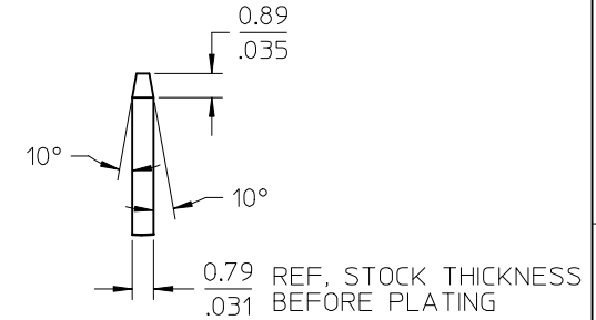
DETAIL ZZ SCALE 5:1
