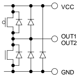
Figure 18. OUT1 / OUT2
