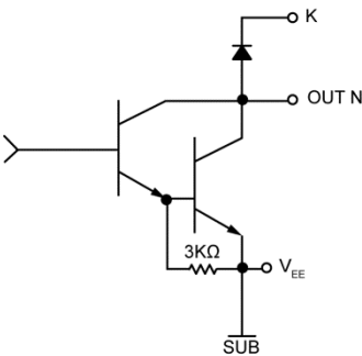
Typical Output Driver
