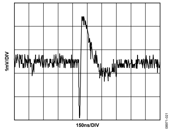
Figure 21. DAC-to-DAC Crosstalk
