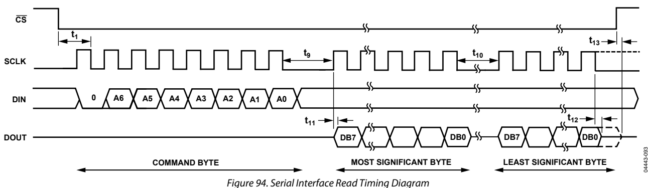
Figure 94. Serial Interface Read Timing Diagram
