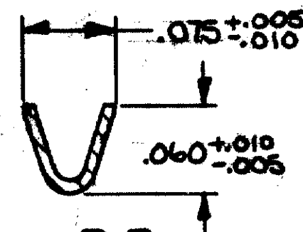
SECT B-B
