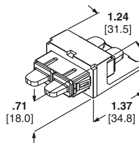
SC Duplex Adapter
