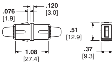
SC Simplex Adapter
