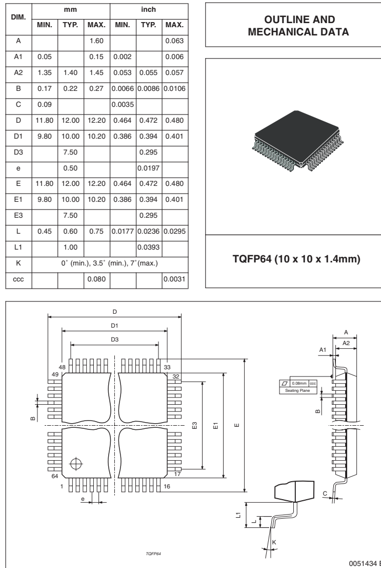
Figure 12. TQFP64 (10 x 10 mm) package dimensions
