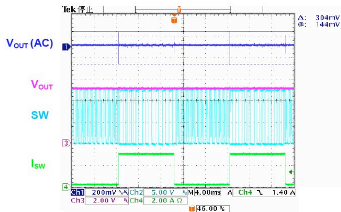
( V_{IN}=12V , V_{OUT}=5V , I_{OUT}=0.1\sim 3A )
