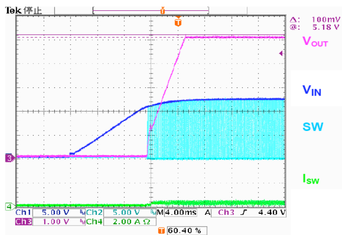
( V_{IN}=12V , V_{OUT}=5V , I_{OUT}=0.2A )
