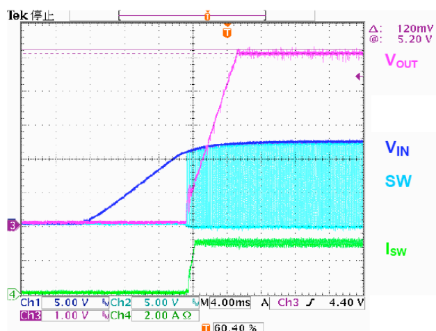
( V_{IN}=12V , V_{OUT}=5V , I_{OUT}=3A )
