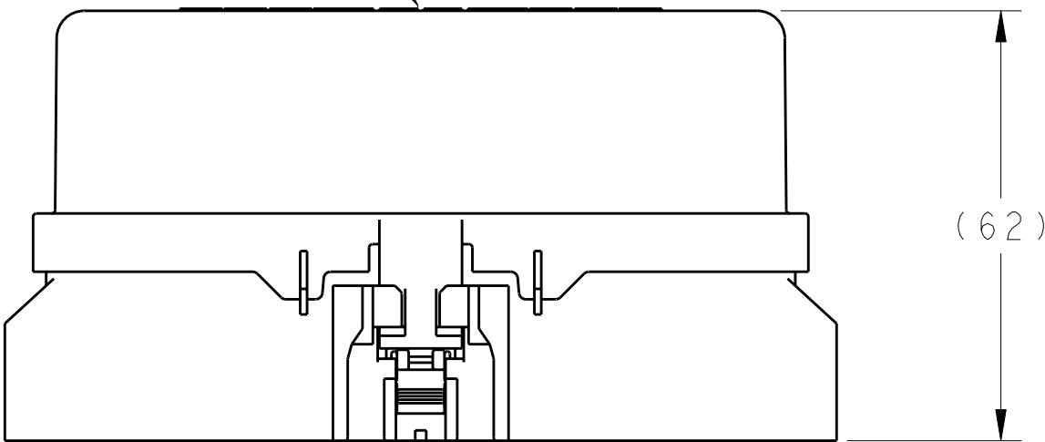
VIEW FOR REFERENCE ONLY (COVER NOT INCLUDED) SCALE 1:1
