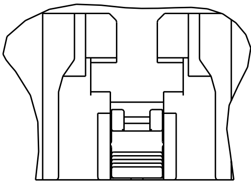
CPA OPEN POSITION (AS SHIPPED)
