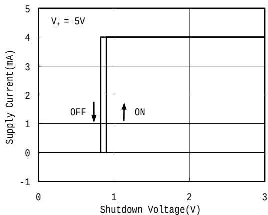
Supply Current vs.Shutdown Voltage
