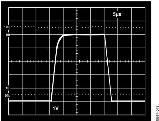
Figure 48. Pulse Response of In-Amp to a 500 mV p-p Input Signal; V S = 5 V, 0 V; Gain = 0
