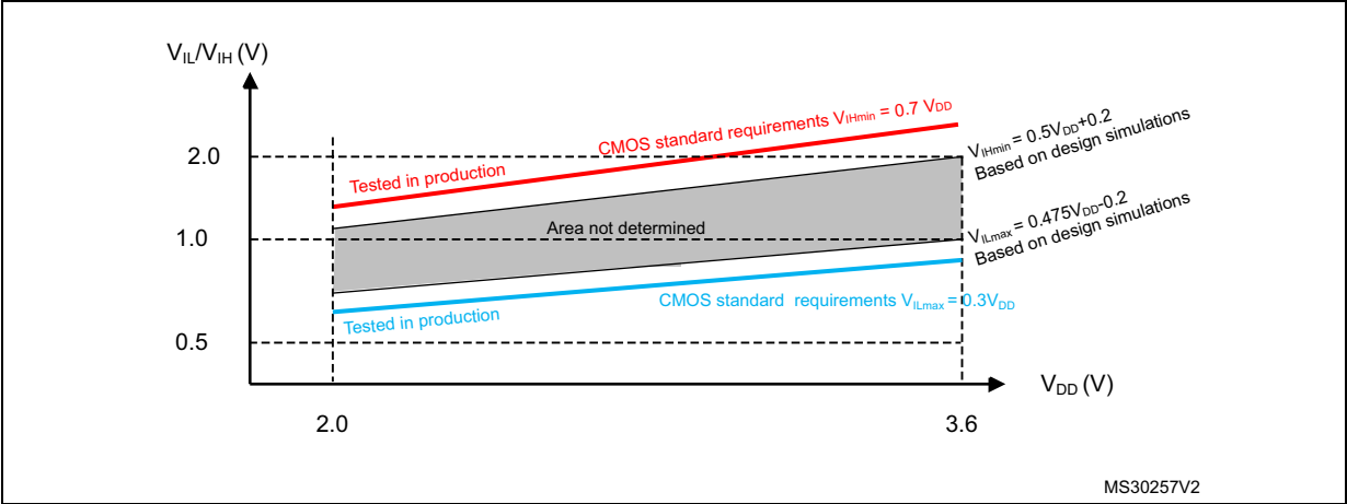
Figure 21. Five volt tolerant (FT and FTf) I/O input characteristics - CMOS port
