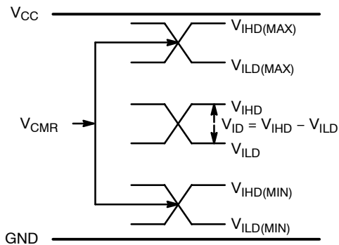
Figure 8. V_{CM} Diagram
