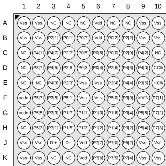
Figure 8. CY8C24094 OCD (Not for Production)
