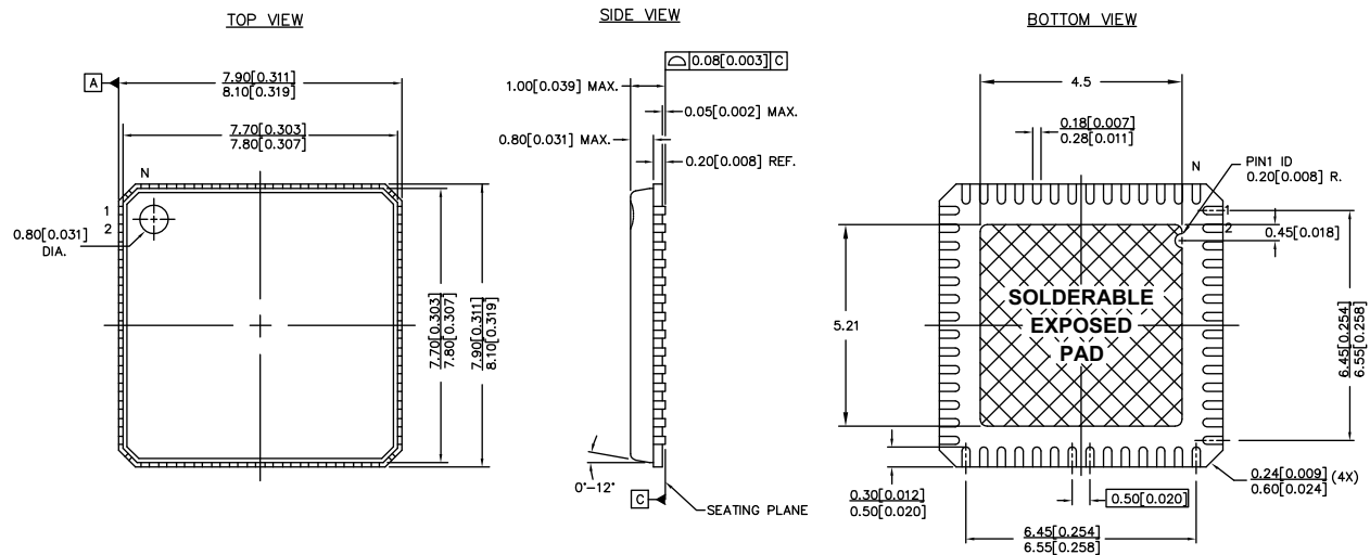
Figure 16. 56-Pin (8 × 8 mm) QFN
