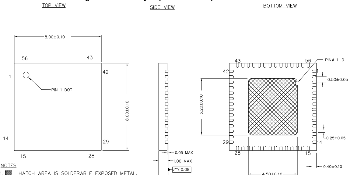
Figure 17. 56-Pin QFN (8 × 8 × 0.9 mm) – Sawn
