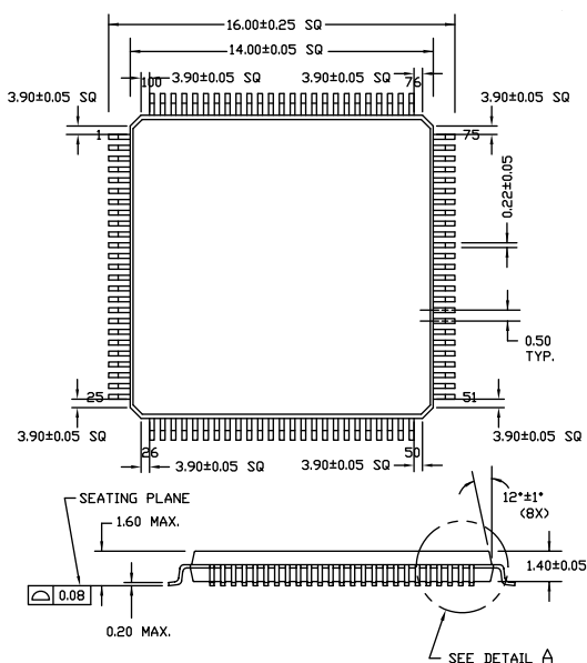
Figure 20. 100-Pin (14 × 14 × 1.4 mm) TQFP
