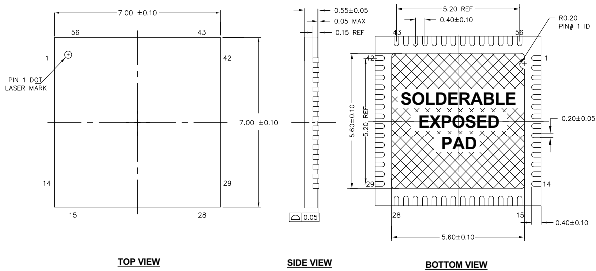
Figure 15. 56-Pin ( 7 \times 7 \times 0.6 mm) QFN
