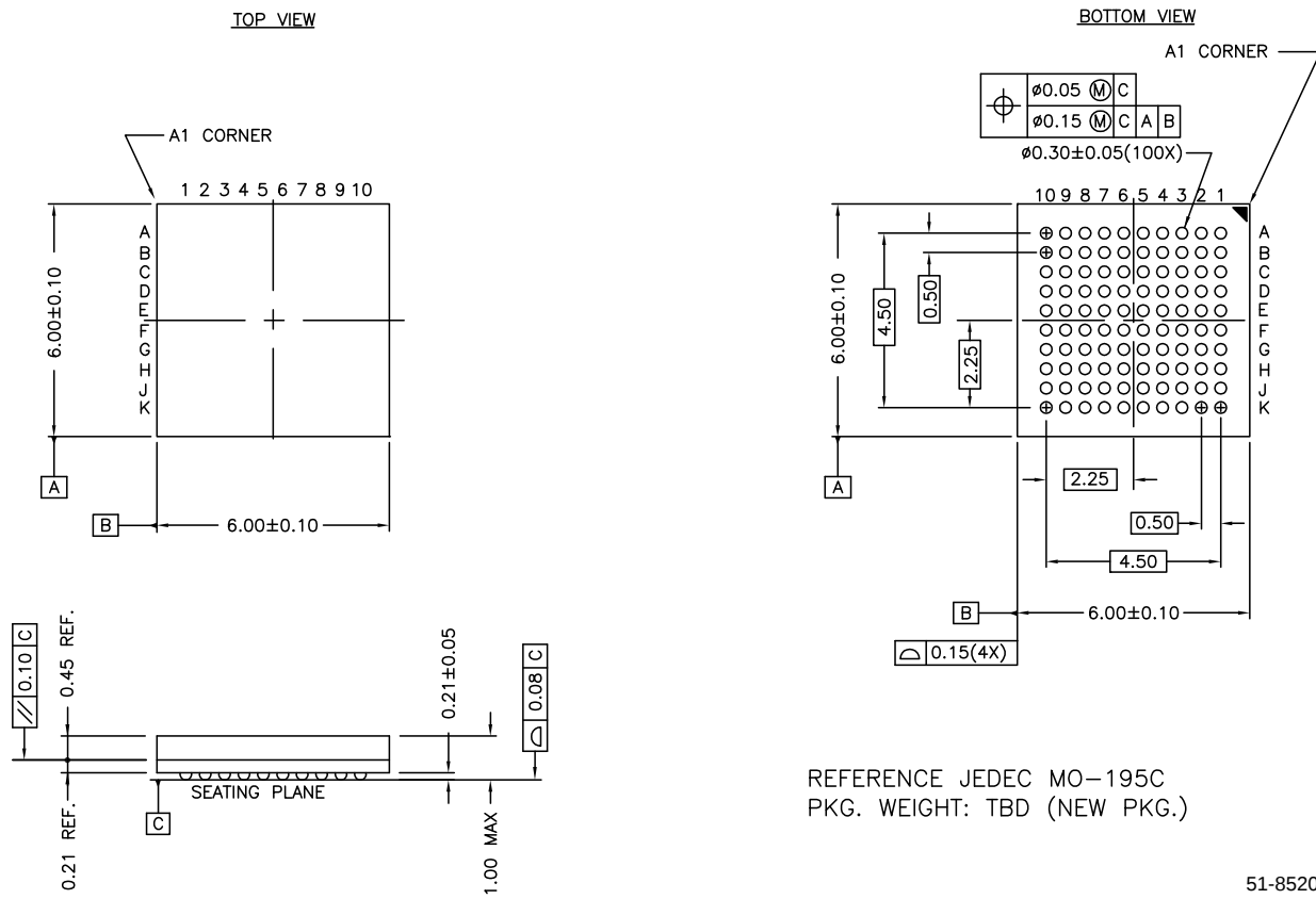
Figure 19. 100-Ball (6 × 6 mm) VFBGA
