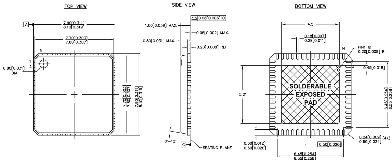
Figure 16. 56-Pin (8 × 8 mm) QFN
