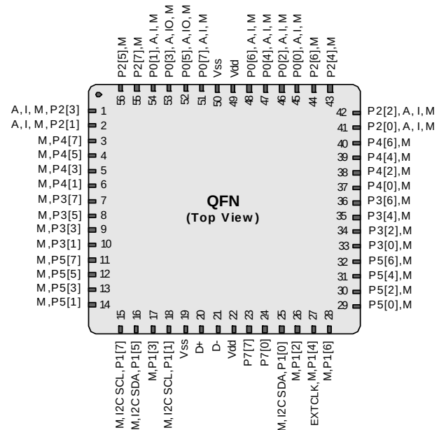
Figure 3. CY8C24794 56-Pin PSoC Device [3]
