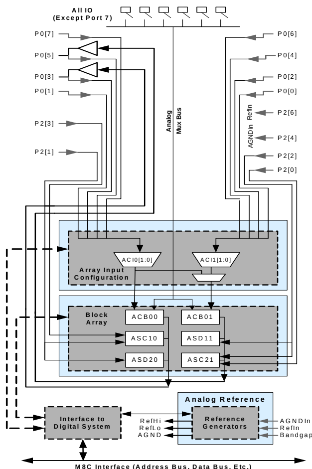
Figure 2. Analog System Block Diagram
