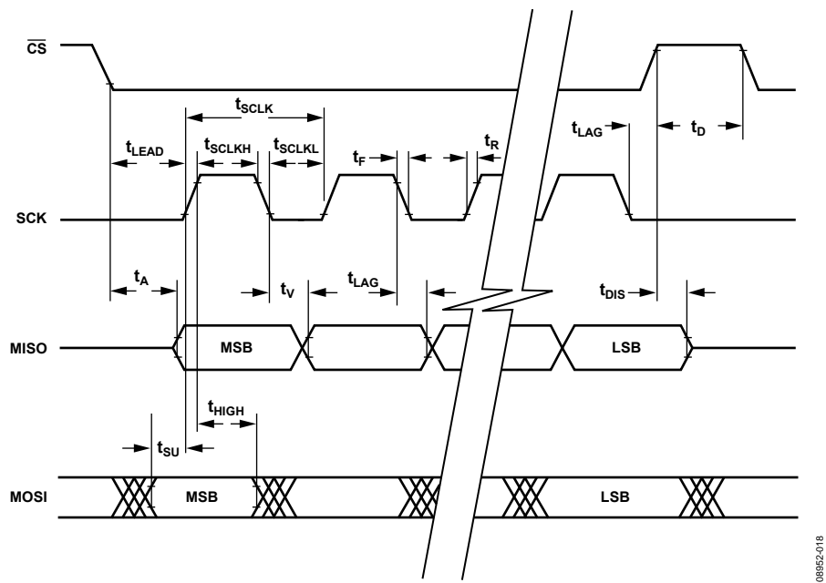
Figure 25. SPI Timings
