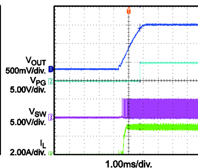
Power Good On with 3A Load
