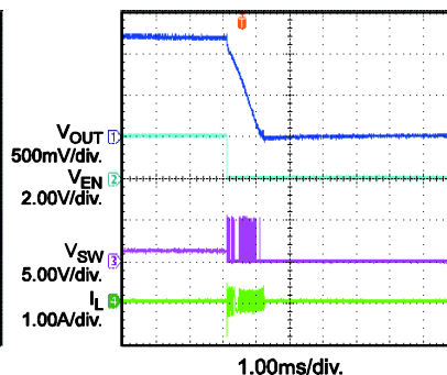
EN Shut Down without Load
